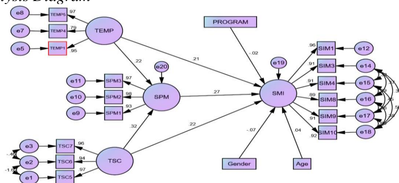
Path Analysis Diagram
