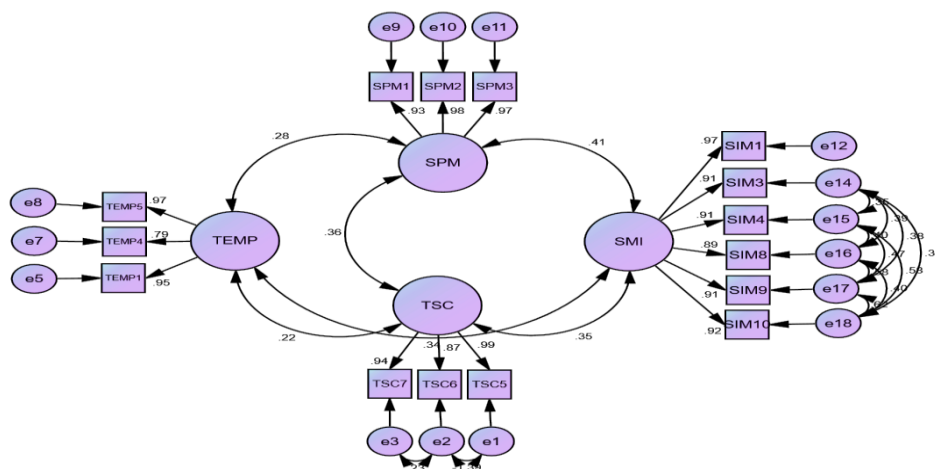
Confirmatory Factor Analysis diagram
