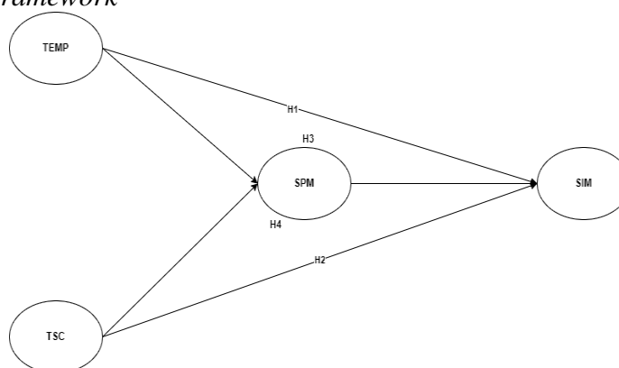
Conceptual Framework
